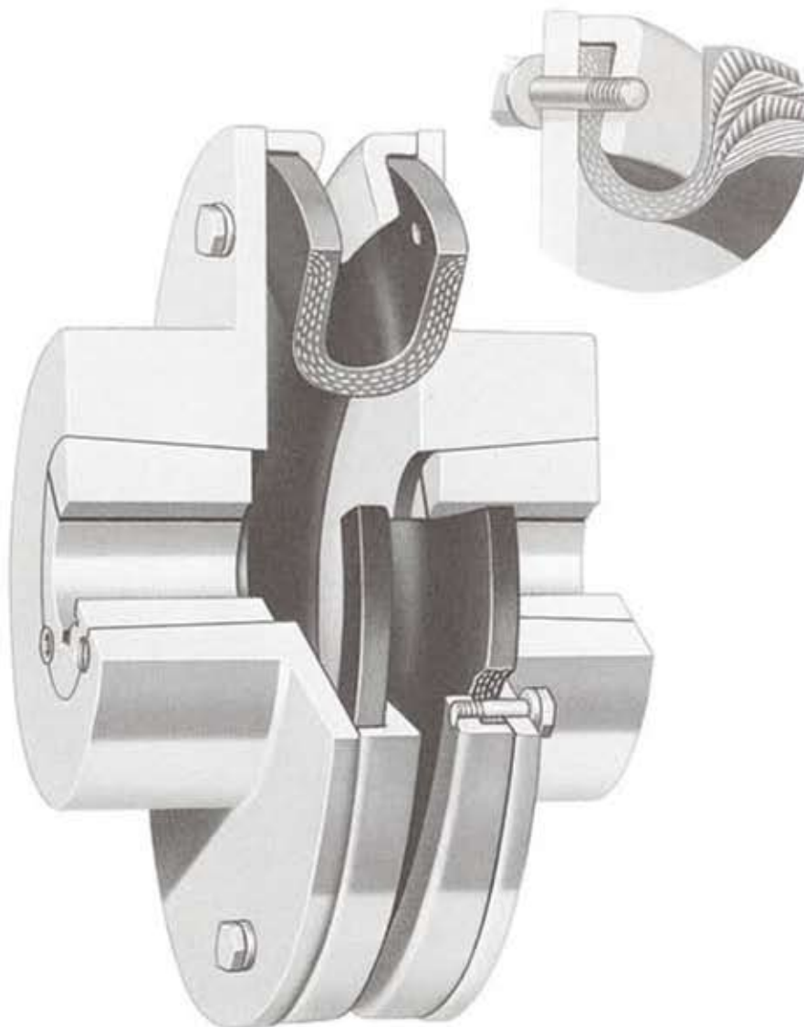
Hub types
